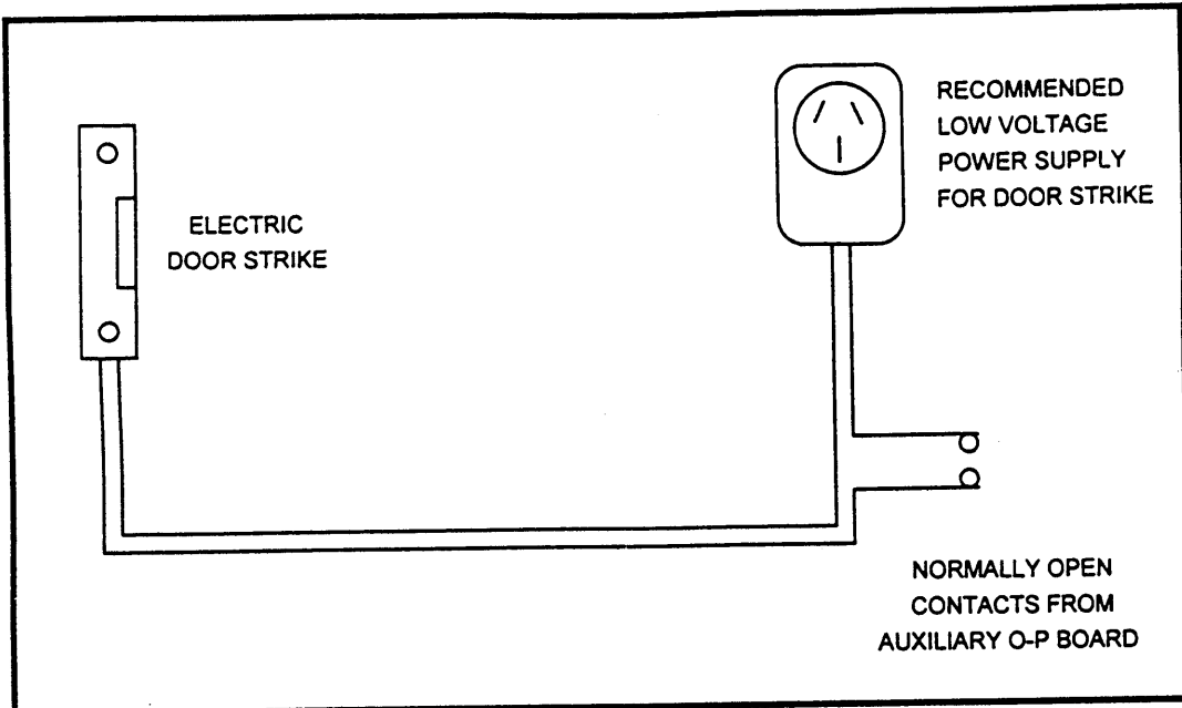
ELECTRIC DOOR STRIKE
